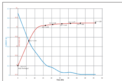
Graph for SMPS cum Battery Charger 24V 03A
