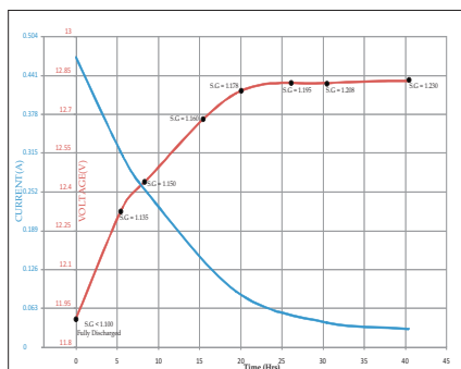
Graph for SMPS cum Battery Charger 12V 03A
