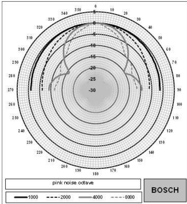
Polar diagram LC1-PC20G6-6-IN high frequency part (frequency in Hz)
