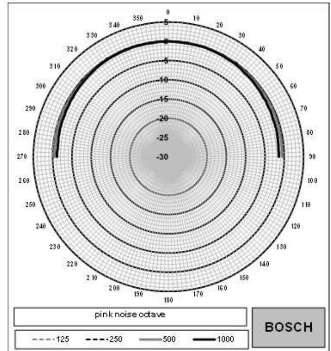
Polar diagram LC1-PC20G6-6-IN low frequency part (frequency in Hz)
